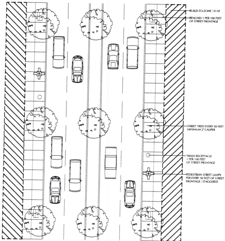
HOTEL STREET AT CADIZ STREET AND PRIMARY STREET
