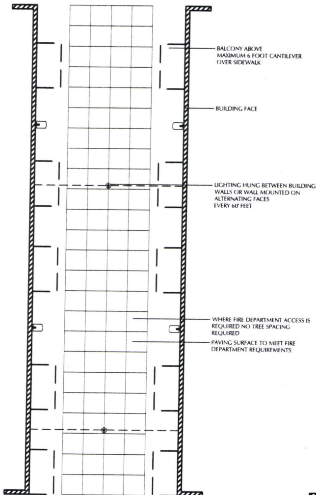
MEWS / PEDESTRIAN WAY WITH FIRE DEPARTMENT ACCESS 2067-298
