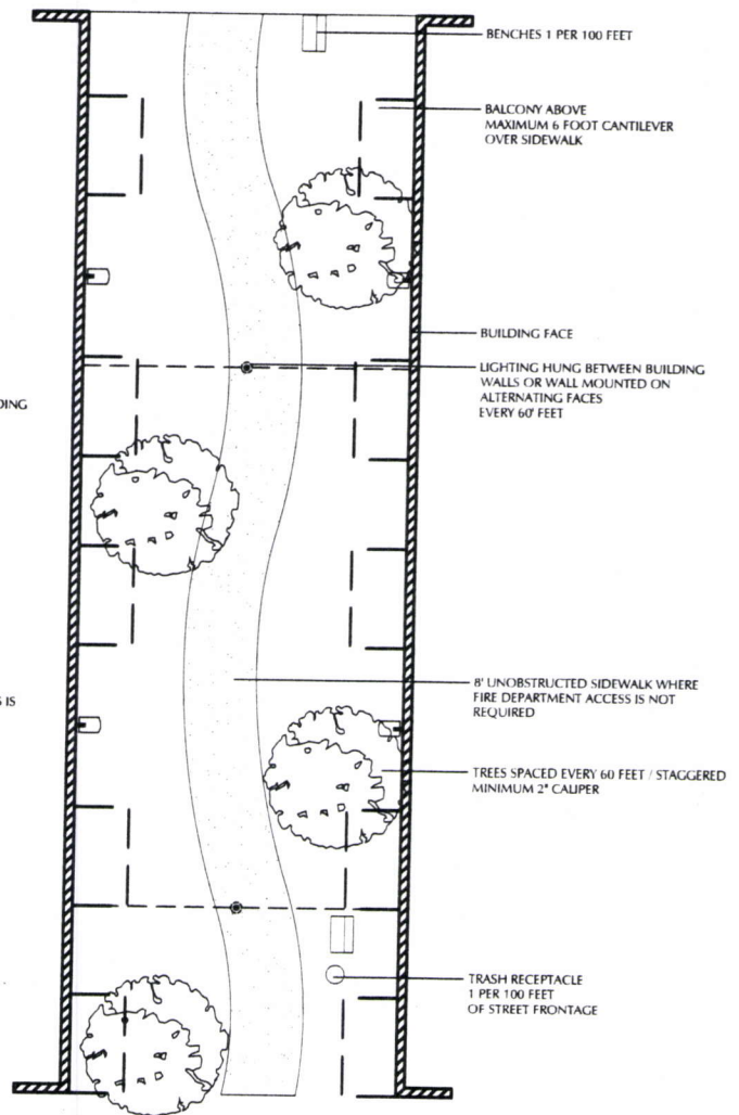
MEWS / PEDESTRIAN WAY WITHOUT FIRE DEPARTMENT ACCESS
